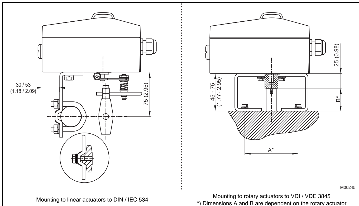
Fig. 11: Mounting drawings
