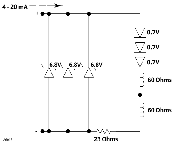
Figure 1. Equivalent Circuit
